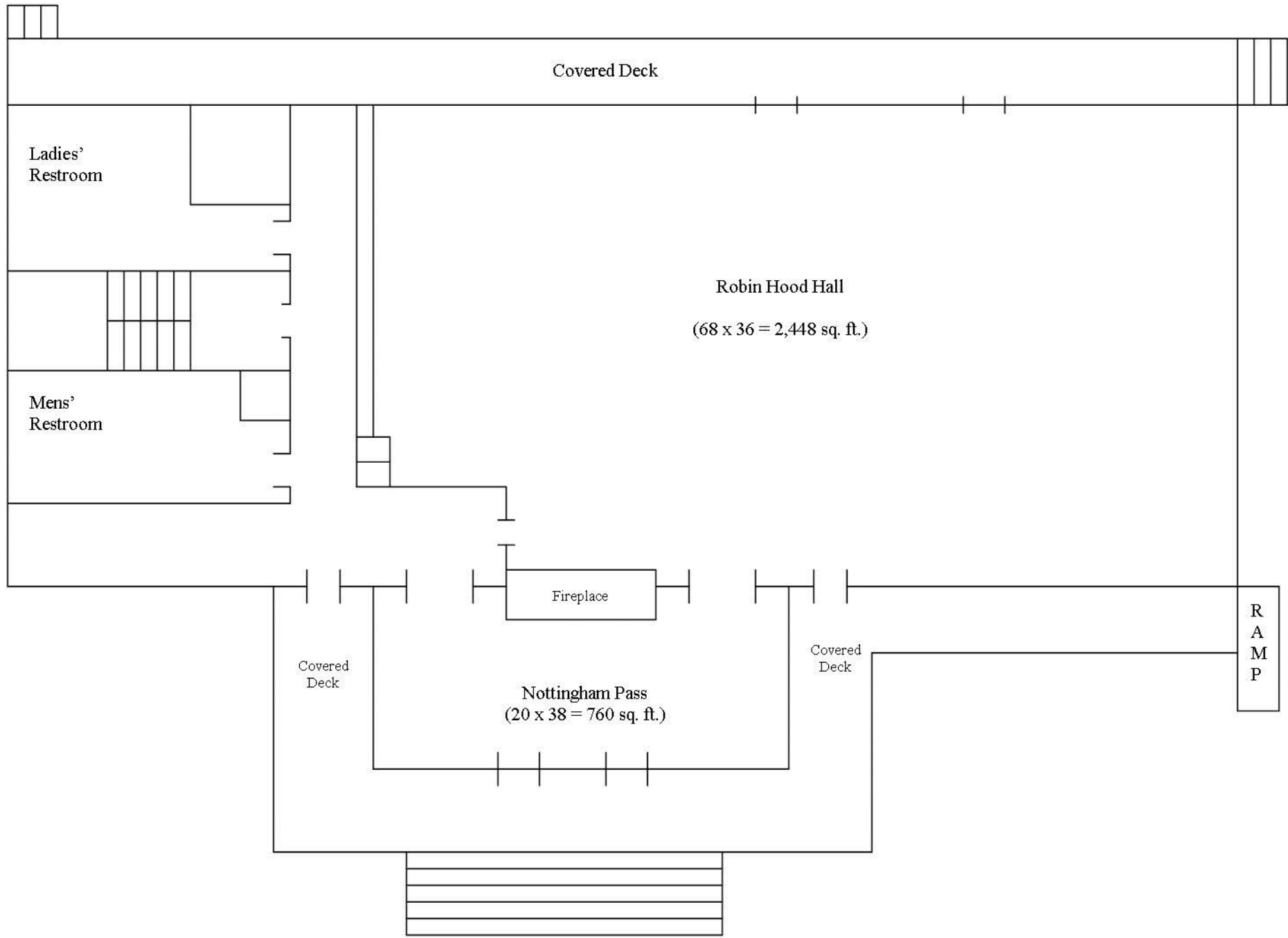
Sherwood Forest Resort Conference Center—Main Level Floor Plan
